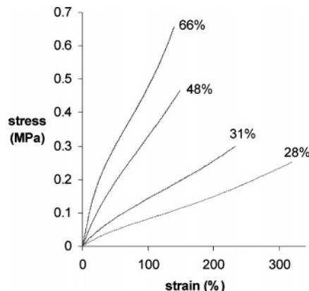
Figure 8. Sample tensile data for bulk films containing varying amounts of pN 3 Phe.
