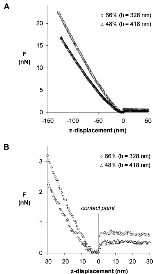
Figure 3. Representative loading indentation profiles for thin films of aE-66%-pN 3 Phe and aE-48%-pN 3 Phe, showing force vs indentation depth (z-displacement). (A) shows the entire profiles; (B) is magnified to show the contact point assignment.
