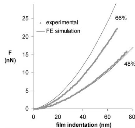
Figure 7. Superposition of experimental AFM data and finite element simulations of indentation based on bulk tensile data for thin films of aE-66%-pN 3 Phe and aE-48%-pN 3 Phe.
