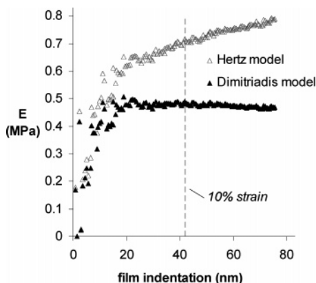
Figure 5. Elastic modulus ( E ) calculated at each point in the AFM indentation using Hertz and Dimitriadis models (eq 1) is shown for an aE-48%-pN 3 Phe film.
