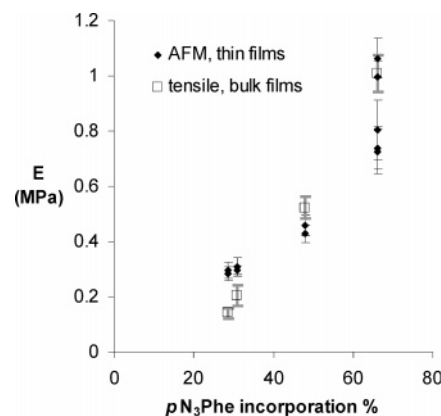
Figure 9. Measured elastic moduli of thin films of aE- pN_3Phe vs fraction replacement of Phe by pN_3Phe . Results from AFM nanoindentation of thin films and tensile testing of bulk films are compared.
