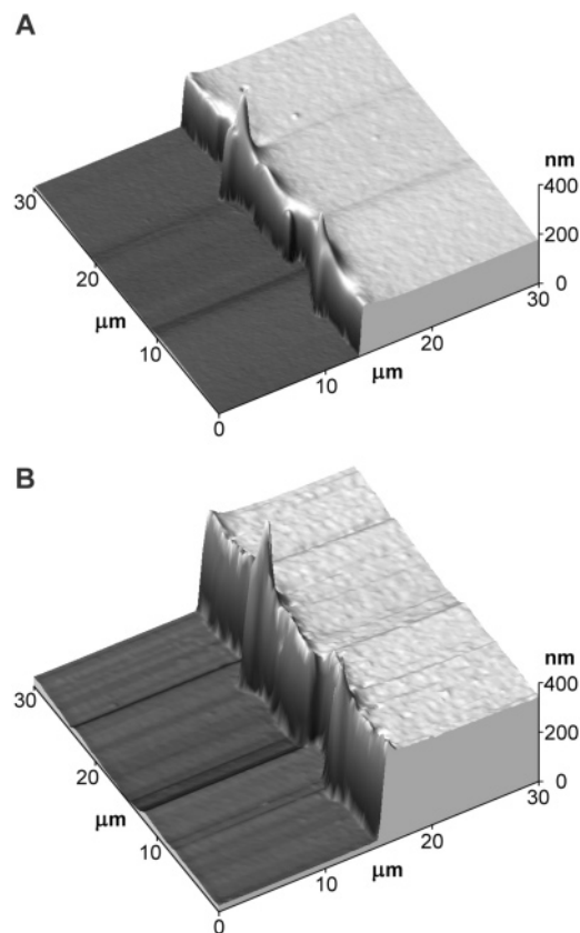
Figure 2. AFM topography scans of cut edges of an aE-48%-pN 3 Phe film, dry (A) and in water (B). The spikes at the edge are artifacts of the scratching procedure.
