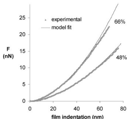
Figure 6. Experimental AFM indentation data compared to Dimitriadis model (eq 1) fits for thin films of aE-66%-pN 3 Phe and aE-48%-pN 3 Phe.
